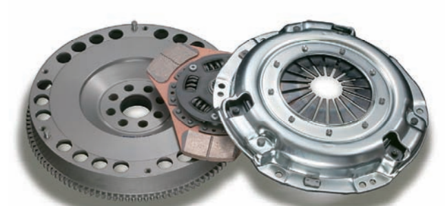
Metallic disc KIT ■26000-3SG-00M
