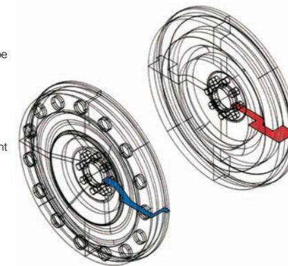
Toda racing chrome molly steel flywheel & a standard flywheel both analytic figures.
